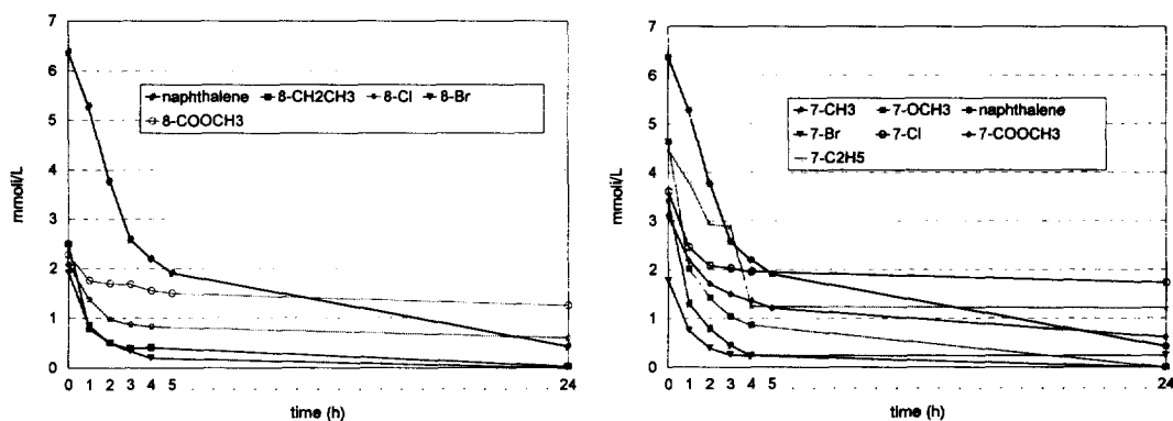
Figure 2 Rate of conversion of 1,2-dihydroxy-1,2-dihydroxynaphthalenes into corresponding 1,2-dihydroxy derivatives
