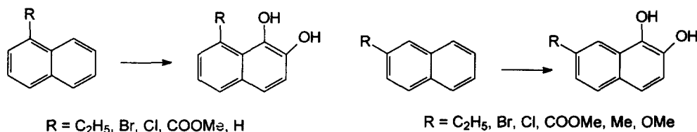
Figure 1 1,2-dihydroxy naphthalenes obtained by bioconversion
